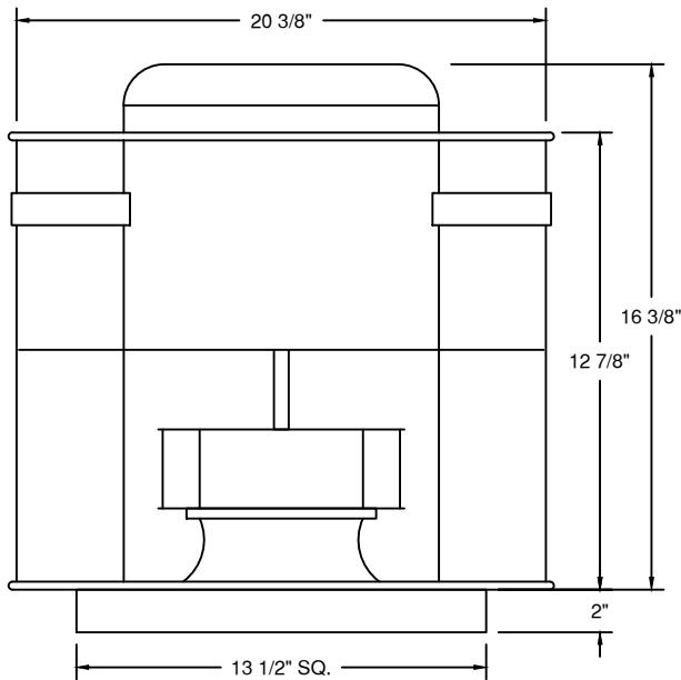
DIMENSIONAL DATA 12" SQ. CURB
